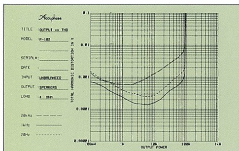
● Power output vs. THD (4-ohm load)
